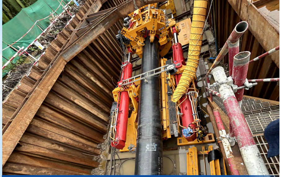
Installation of 36-inch pipeline using the Direct Pipe method in Bangkok, Thailand
